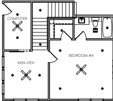
02 2ND FLOOR PLAN
