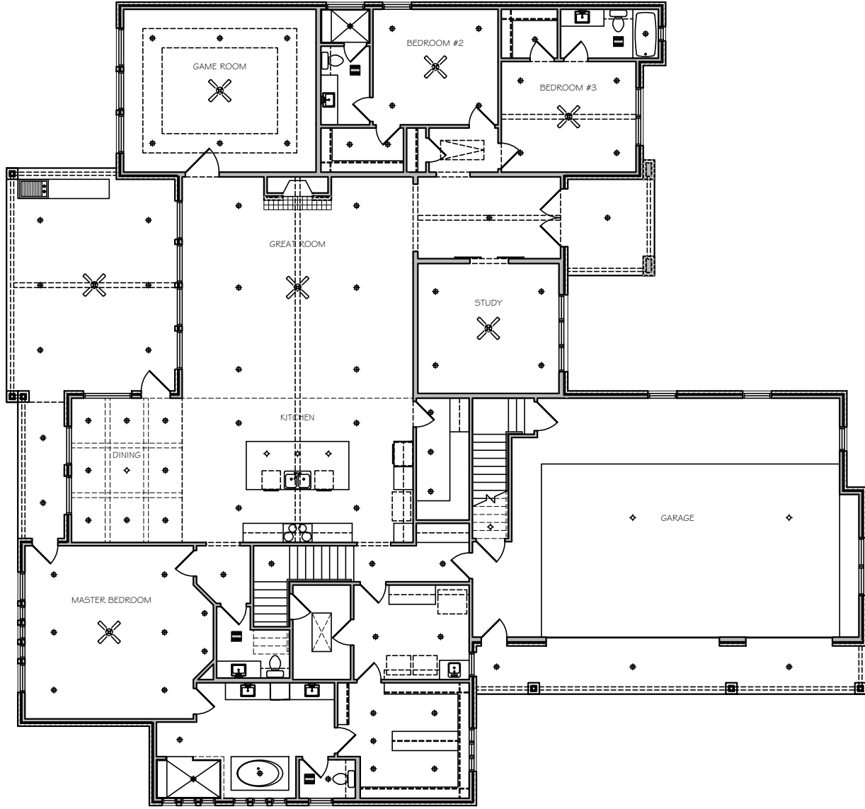
01 1ST FLOOR PLAN
